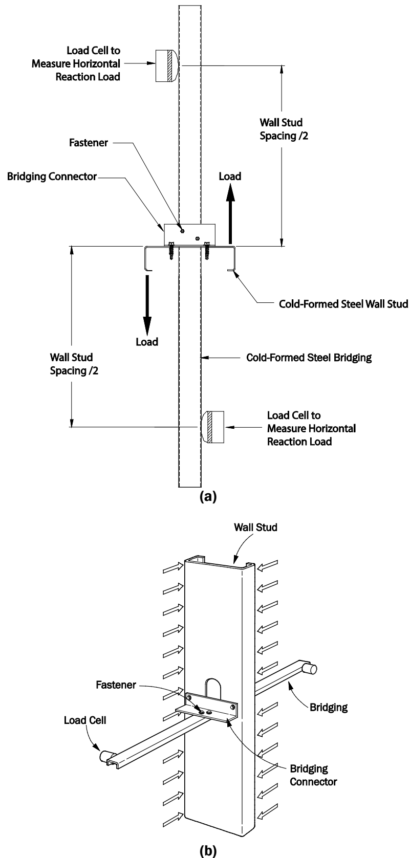
Figure 2 – Rotational Strength Test Setup for Bridging Connector Assembly
